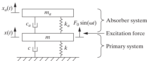
Figure 5.18 A schematic of a vibration absorber with damping in both the primary and absorber system.
